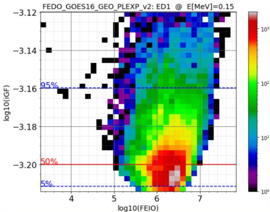
Figure 4: Histogram of the distribution of the geometric factors for ED1, derived using Equation 1. The horizontal lines denote selected percentiles of the geometric factors.
