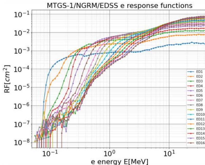
Figure 2: Omni-directional electron response functions of MTG-S1/NGRM Electron Detector (ED) channels.
