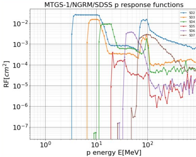
Figure 3: Omni-directional proton response function of MTG-S1/NGRM Stacked Detector (SD) channels.
