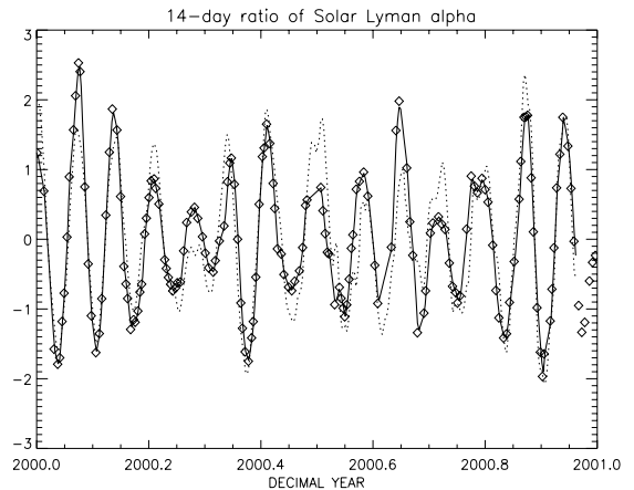
Figure 2. Comparison of the half solar rotation ratio of solar Ly \alpha flux with the SWAN flux ratio index. The abscisse is the decimal year of the data. The dotted line shows the ratio of the Solar Ly \alpha flux measured at D+13.5 divided by the value at D . The thick line shows the predicted ratio using the correlation shown in the previous figure. Both curves are shown in units of normalized ratios as described in the text. The diamonds show the actual dates of SWAN observations. The result obtained for the Solar Ly \alpha flux is quite good. This shows that the total flux emitted by the sun does not change too much over half a solar rotation. The main cause for variation over this period of time is the solar rotation itself.
