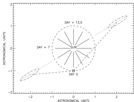
Figure 1. Sketch showing how the solar Ly \alpha flux distribution can be retrieved in every direction. SWAN (position indicated by Day 0) sees the backscattered emission from every direction of space. The region where a large fraction of the photons are scattered (MER) is shown by the small ellipses. Its actual position depends on the density distribution of hydrogen but lies outside of the Earth orbit. Although there is a small parallax effect for values at 90 degrees, the spatial anisotropies of the illuminating flux can be retrieved with sufficient accuracy. We can study the ratio of the values emitted away from SOHO with the one emitted in the direction of SOHO. The value emitted in the direction opposite from SOHO corresponds to the surface of the sun which will be in the center of the visible disk half a solar rotation later (Day + 13.5).
