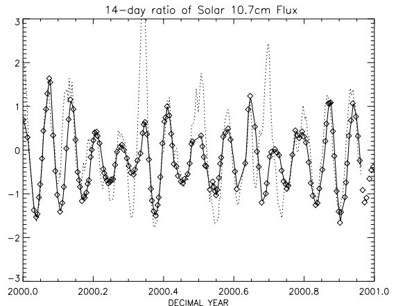
Figure 3. Comparison of the half solar rotation ratio of the 10.7cm solar flux with the SWAN flux ratio. The ordinate is in units of normalized ratio (Ratio value minus mean ratio and divided by standard deviation of ratio). As in the previous figure, the dotted line shows the ratio of the index values measured at date D + 13.5 and D . The thick line shows the predicted ratio using the correlation shown in figure 2. The diamonds show the actual dates of SWAN observations. Here, the comparison is not as good as in the previous case. The amplitude can be significantly different. We even note a phase opposition between the two indices around 2000.7.
