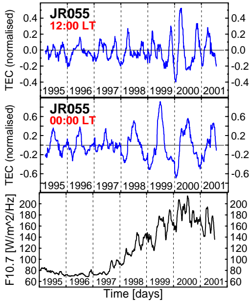
Fig.1 Normalised TEC 31-day running medians, JR055 site.
