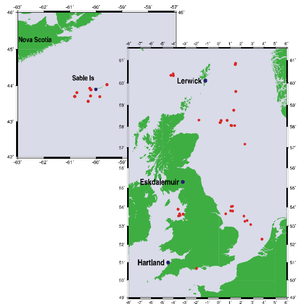
Fig. 5 Locations of oil fields where external field variations have been used to improve drilling accuracy.
